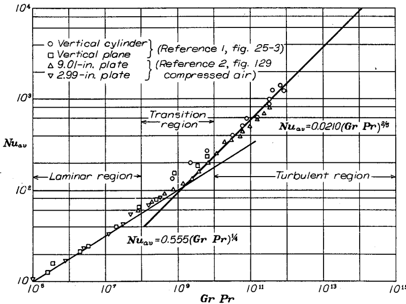
FIGURE 4.—Average Nusselt number for free-convection flows on a vertical plate. Experimental data from references 1 and 2.
