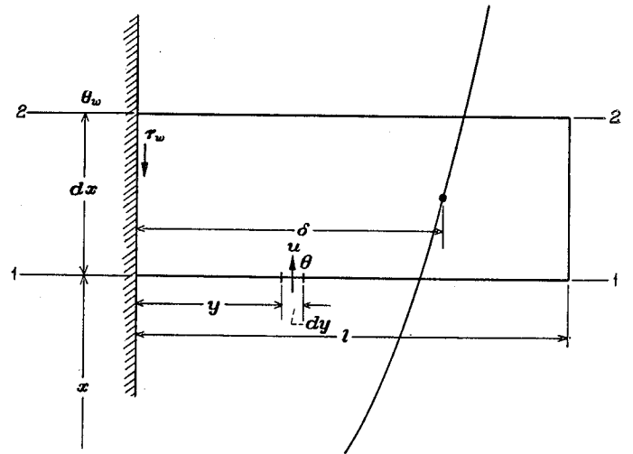
FIGURE 1.—Nomenclature in deriving equations for free-convection boundary layer.
